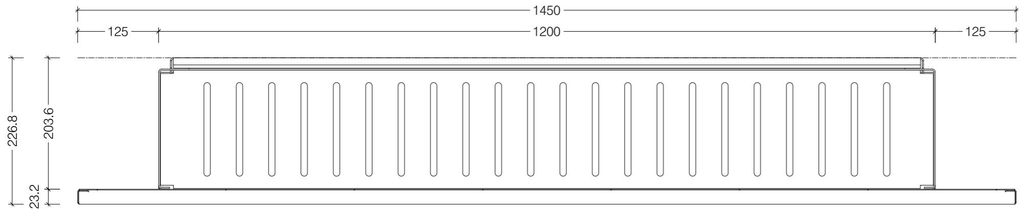
Top View
