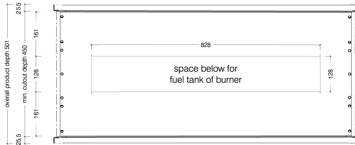
Top View
