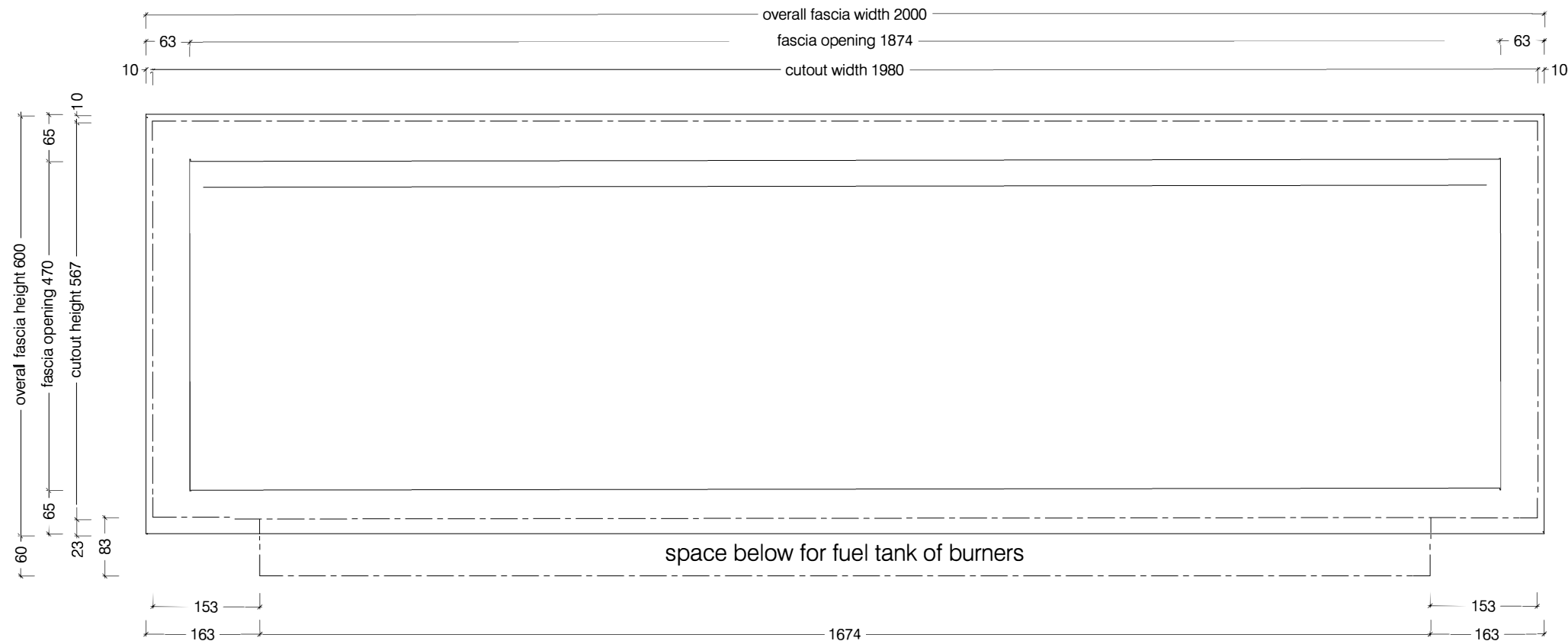
Front View
