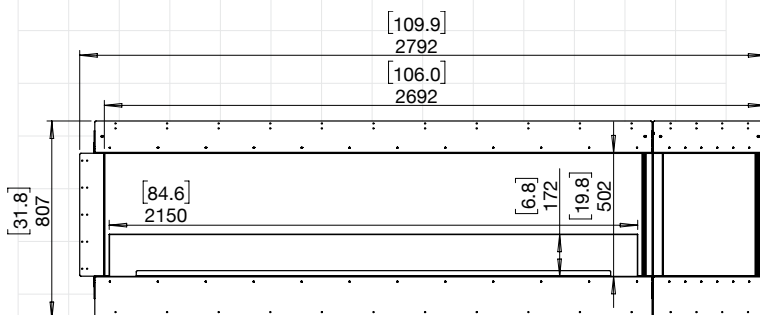
104RC.BXR (RIGHT DECORATIVE BOX)
