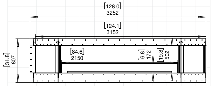
122RC.BX2 (LEFT & RIGHT DECORATIVE BOXES)
