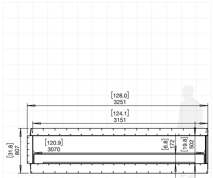
122RC (FLAME ONLY)
