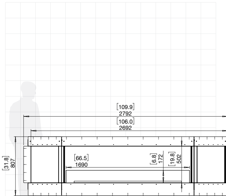
104RC.BX2 (LEFT & RIGHT DECORATIVE BOXES)
