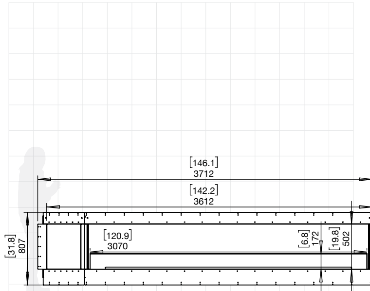
140RC.BXL (LEFT DECORATIVE BOX)
