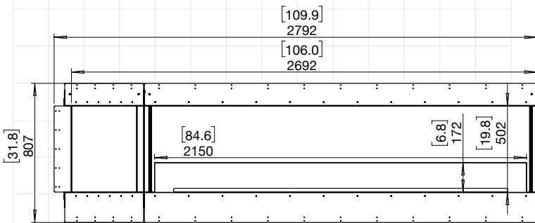
104RC.BXL (LEFT DECORATIVE BOX)
