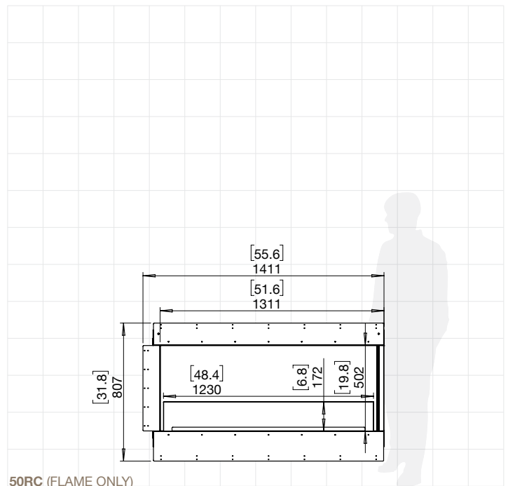
50RC (FLAME ONLY)
