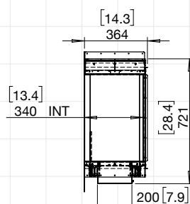
104RC.BXR (RIGHT DECORATIVE BOX)
